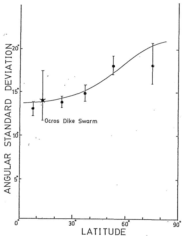
Fig.3-18a Angular standard deviation of Ocos dike swarm VGPs and the global trend of the last 5Ma summarized for each 15° latitude strips by McElhinny and Merrill (1975). Error bars indicate 95% confidence intervals.
