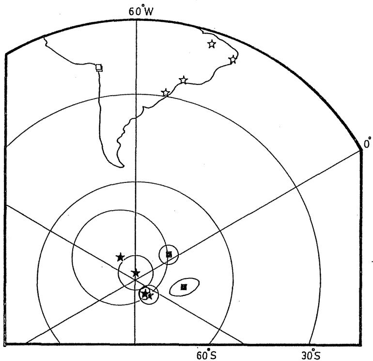
Fig.4-21 Paleomagnetic poles of Cretaceous rock formations in the northernmost Chile (squares) and the stable platform (stars) and their 95% confidence circles/ovals. Corresponding sampling localities are shown as small open symbols in the map.
