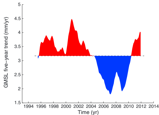
Figure 1. Temporal evolution of the GMSL rate computed over 5 year long moving windows. The horizontal line represents the average rate of 3.2 mm/yr from 1994 to 2014. The red and blue areas indicate the fast and slow rates with respect to the average rate, respectively. The GMSL rate behavior was fast from 1996 to 2004, slow from 2005 to 2010, and then fast again.
