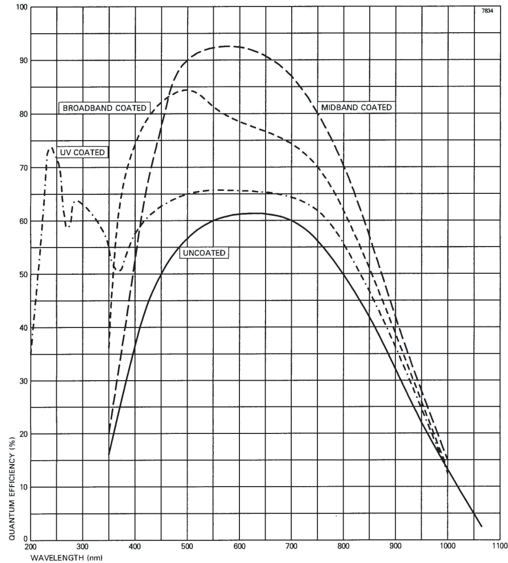
TYPICAL SPECTRAL RESPONSE (At -20^{\circ}\text{C} , no window)
