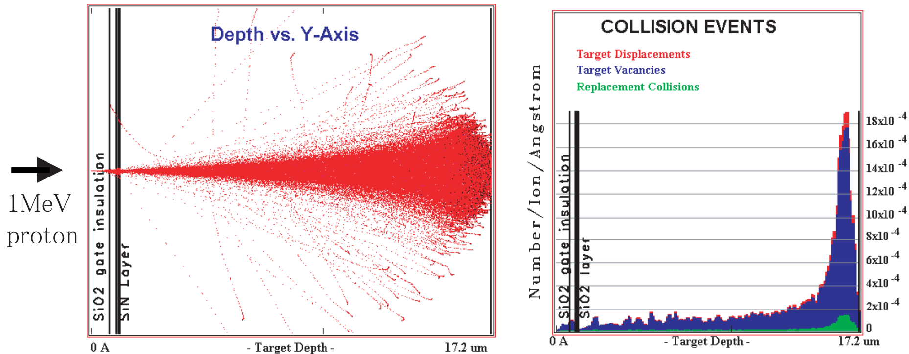
Fig.5.3: The Monte Carlo simulation result by TRIM. CCD47-20 is calculated as a target which consists of substances of six layers. The proton energy which gives the maximum damage is about 1 MeV. Left: Ranges at the simulation of irradiating 10000 1MeV protons perpendicularly from the front of CCD, Right: The situation of the damage caused to CCD.
